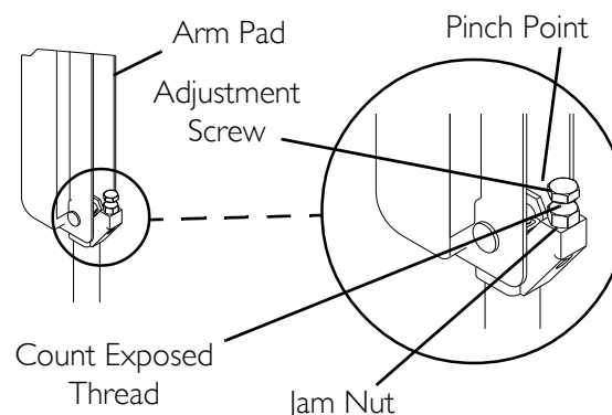
FIGURE 7.3 Adjusting Angle
