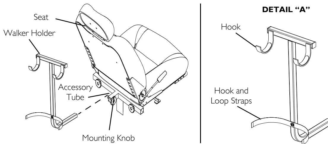
FIGURE 14.3 Installing/Removing/Using the Walker Holder
