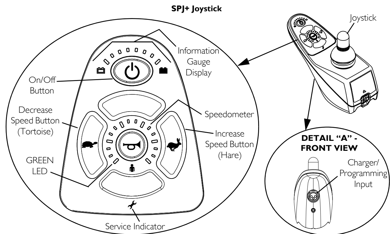
FIGURE 6.3 SPJ™ + Joystick Switches and Indicators
