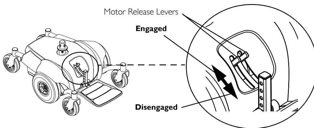
FIGURE 11.2 Engaging/Disengaging Motor Release Lever
