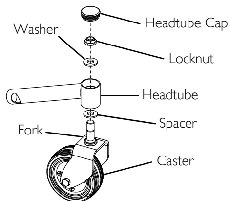
FIGURE 11.4 Adjusting Forks
