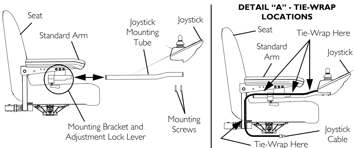
FIGURE 12.1 Removing/Installing the Joystick
