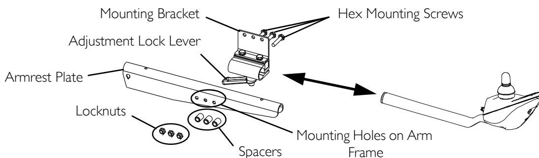
FIGURE 12.2 Repositioning the Joystick
