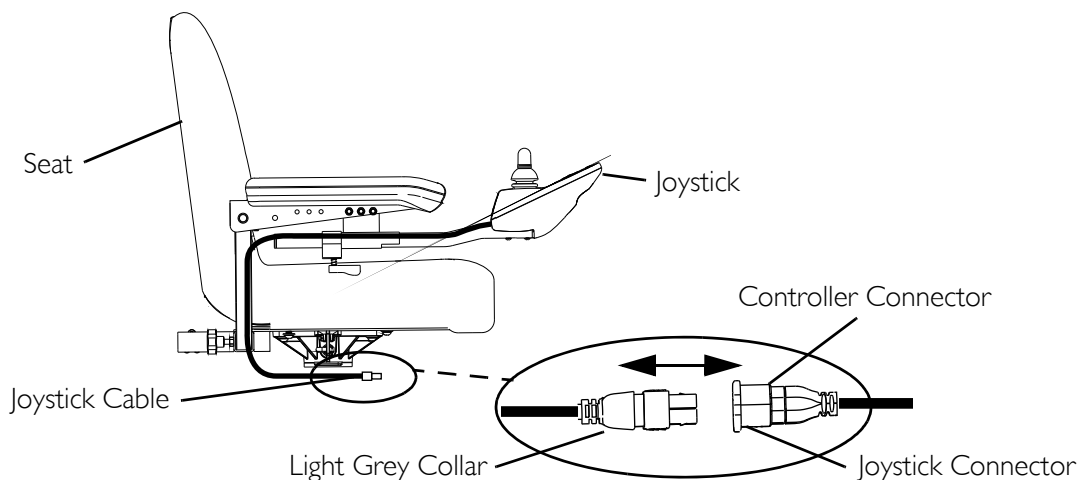
FIGURE 12.3 Disconnecting/Connecting the Joystick
